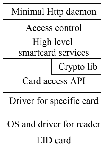
Figure 2: Architecture of the local http server
